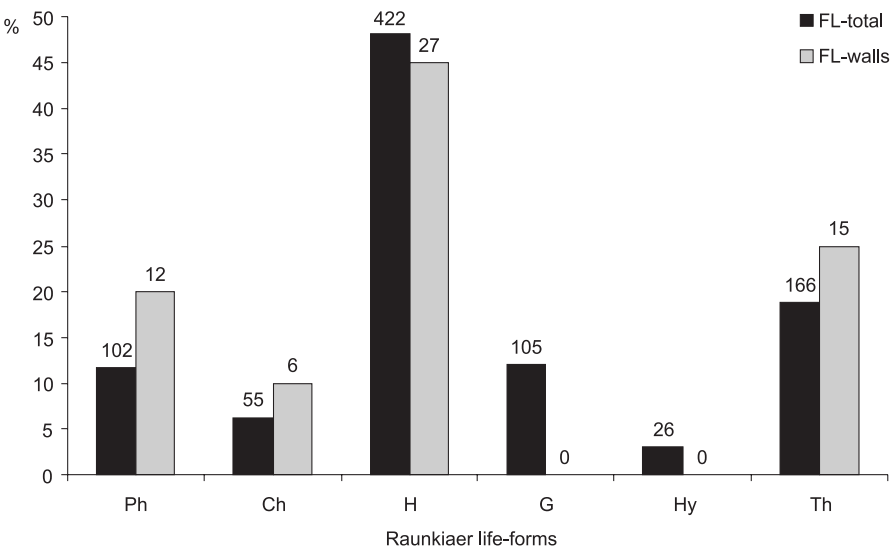
Fig. 72. Spectrum of Raunkiaer life-forms on walls (FL-walls) and in the total flora (FL-total) Explanations: see Fig. 16
