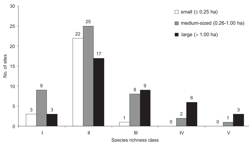
Fig. 24. Distribution of species richness at West Slavic archaeological sites
