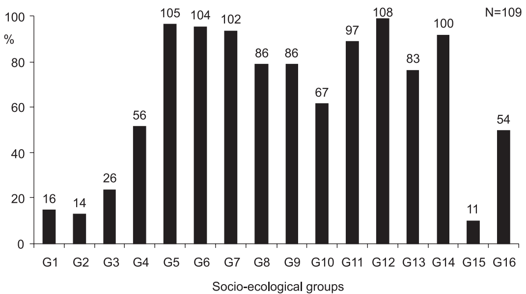
Fig. 21. Importance of socio-ecological groups in the studied vegetation, expressed as the number of West Slavic archaeological sites where they were recorded Explanations: see section 4.3.4
