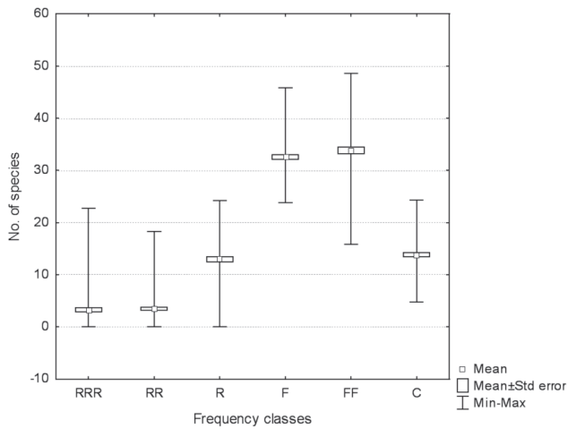
Fig. 29. Mean values and ranges of species number within frequency classes at West Slavic sites Explanations: see Table 1
