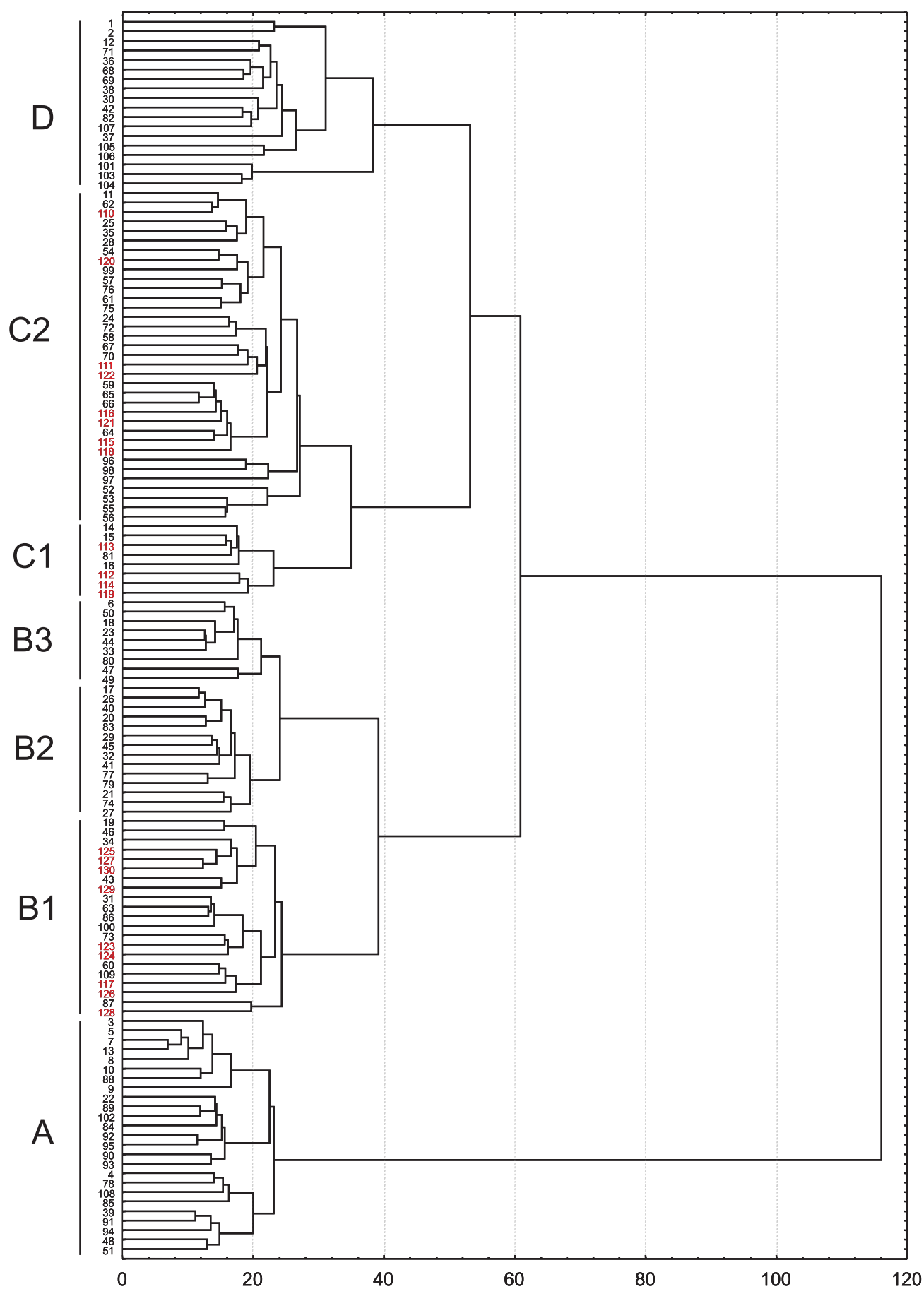
Fig. 51. Dendrogram of species number and abundance at individual sites, constructed on the basis of Euclidean distances by agglomerative clustering (Ward method) for 130 sites
