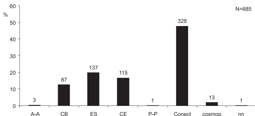
Fig. 15. Contributions of geographic elements and sub-elements to the native flora of West Slavic archaeological sites
