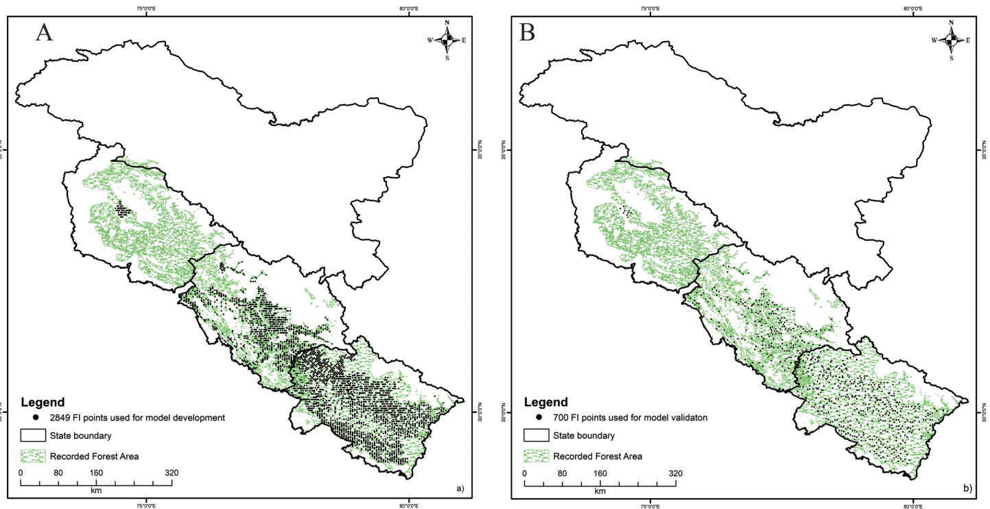
Fig. 2. Distribution of 2849 forest inventory (FI) points used for Forest Biodiversity Index model development (A) and 700 randomly selected FI points used for validation (B)
